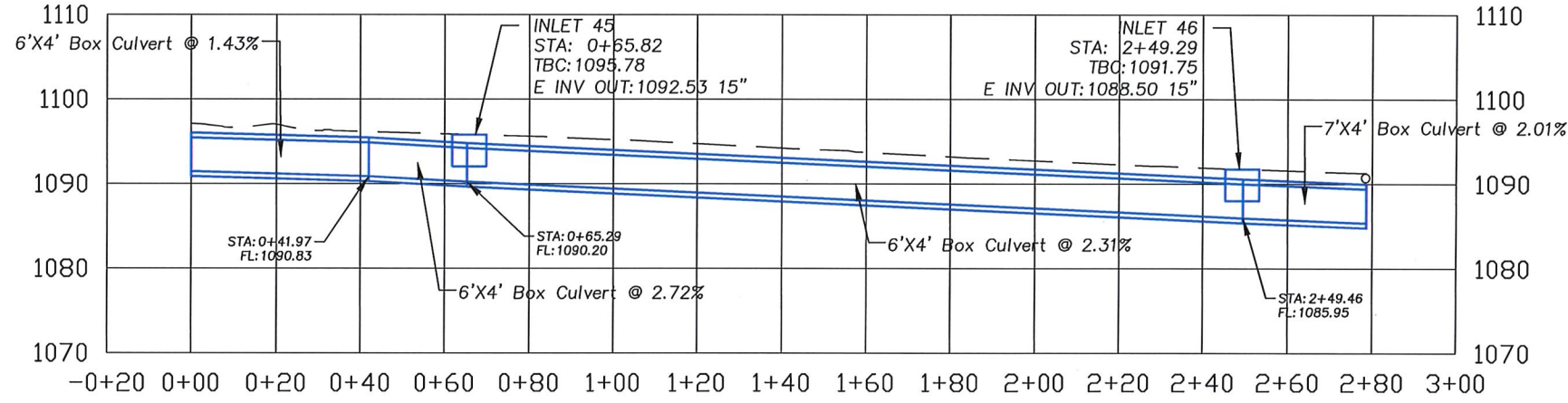
2 ROLLA STREET STORM PROFILE - Rolla St from 7th St to 8th St Scale: 1" = 40' H 1" = 20' V
