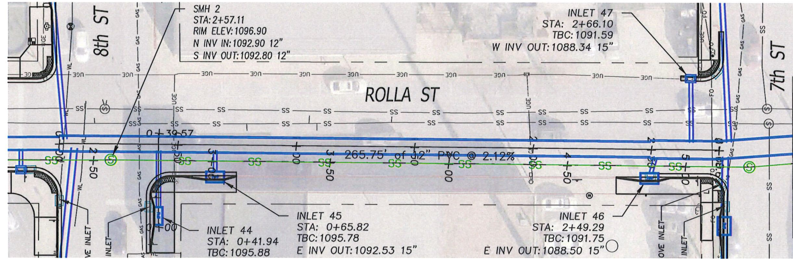
1 ROLLA STREET STORM PLAN - Rolla St from 7th St to 8th St Scale: 1" = 40' H
