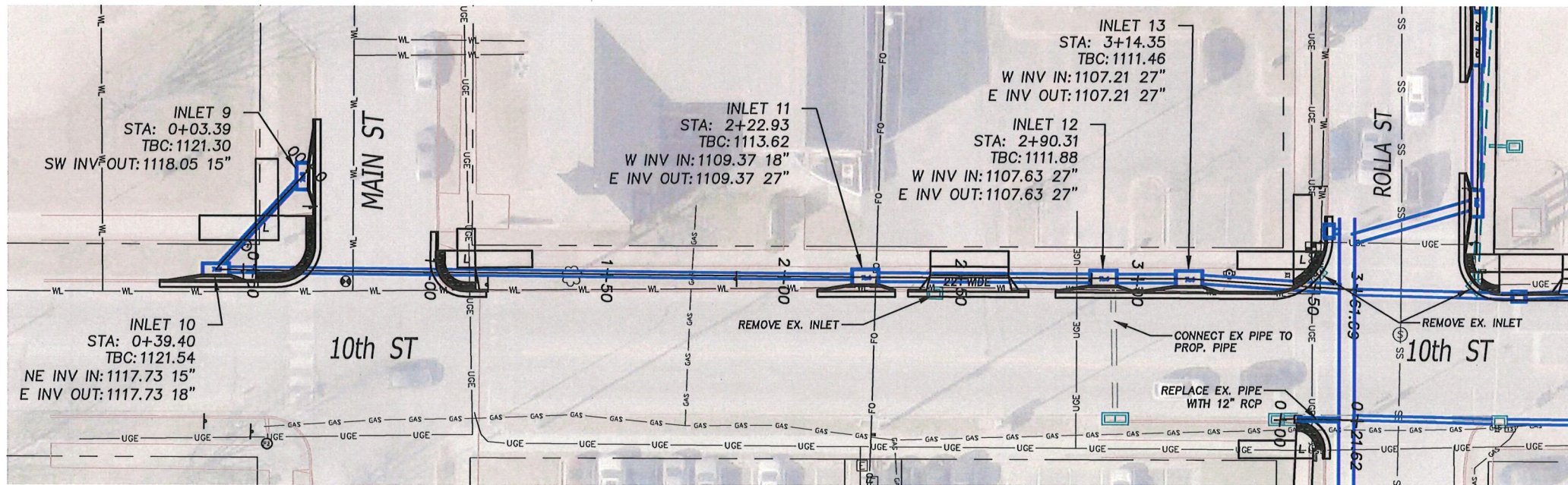
1 ROLLA STREET STORM PLAN - 10th St from Main St to Rolla St 3 Scale: 1" = 40' H
