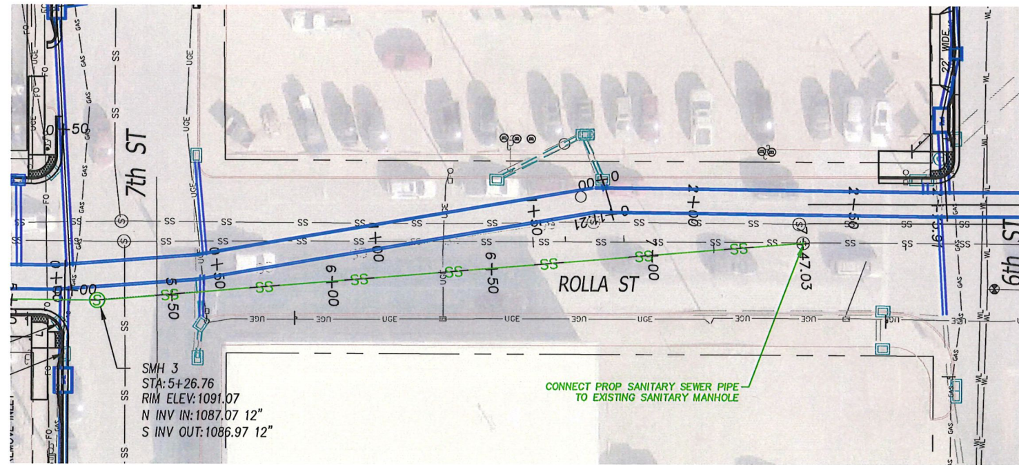
1 ROLLA STREET STORM PLAN - Rolla St from 6th St to 7th St 13 Scale: 1" = 40' H
