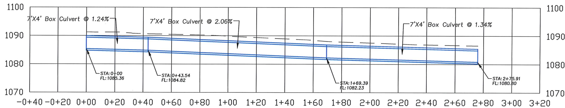
2 ROLLA STREET STORM PROFILE - Rolla St from 6th St to 7th St 13 Scale: 1" = 40' H 1" = 20' V
