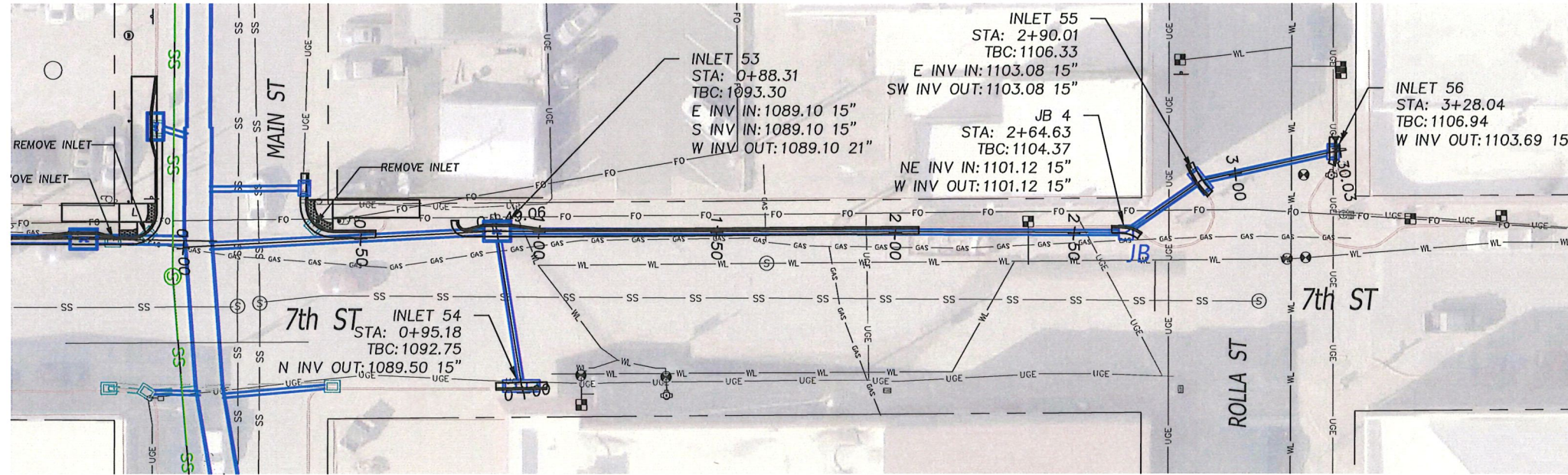
1 ROLLA STREET STORM PLAN - 7th St from Rolla St to Main St 12 Scale: 1" = 40' H
