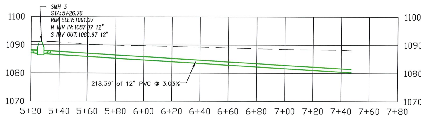
3 ROLLA STREET SANITARY PROFILE - Rolla St from 6th St to 7th St 13 Scale: 1" = 40' H 1" = 20' V
