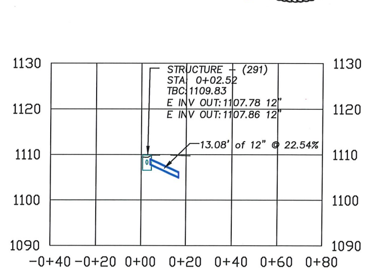
3 ROLLA STREET STORM PROFILE - 10th St & Rolla St SW Curb Return 3 Scale: 1" = 40' H 1" = 20' V
