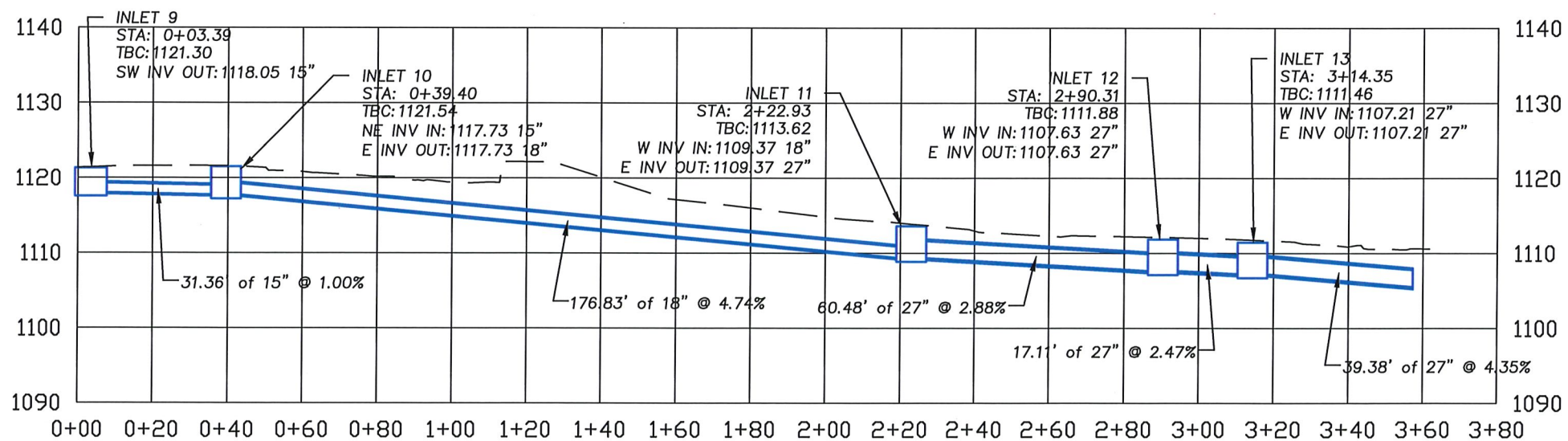
2 ROLLA STREET STORM PROFILE - 10th St from Main St to Rolla St 3 Scale: 1" = 40' H 1" = 20' V
