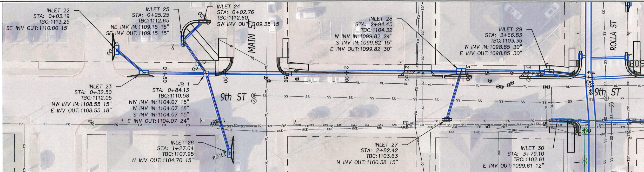
1 ROLLA STREET STORM PLAN - 9th St from Main St to Rolla St Scale: 1" = 40' H
