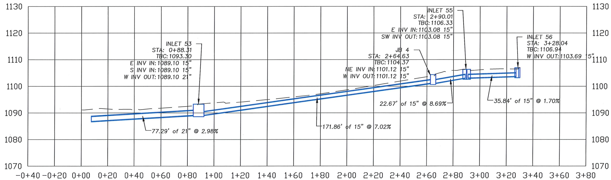
2 ROLLA STREET STORM PROFILE - 7th St from Rolla St to Main St 12 Scale: 1" = 40' H 1" = 20' V
