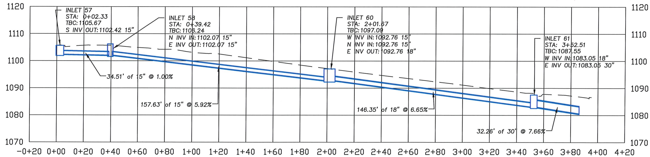
2 14 ROLLA STREET STORM PROFILE - 6th St from Rolla St to Main St Scale: 1" = 40' H 1" = 20' V
