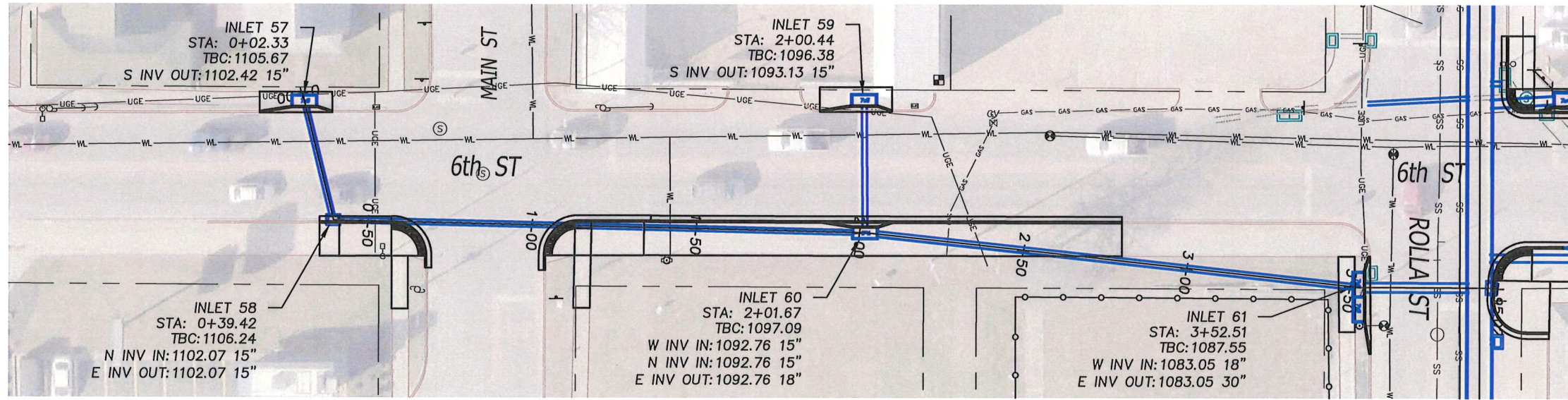
1 14 ROLLA STREET STORM PLAN - 6th St from Rolla St to Main St Scale: 1" = 40' H
