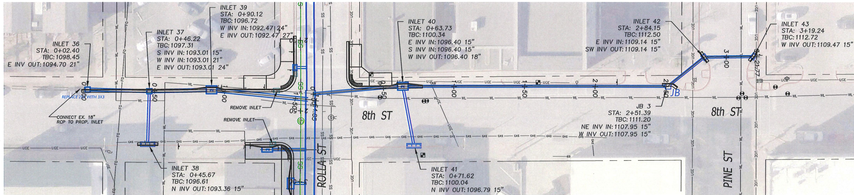
1 9 ROLLA STREET STORM PLAN - 8th St from Rolla St to Pine St Scale: 1" = 40' H
