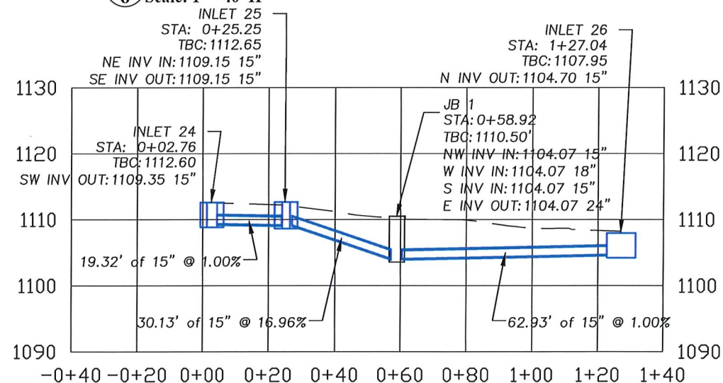
3 ROLLA STREET STORM PROFILE - 9th St and Main St Scale: 1" = 40' H
