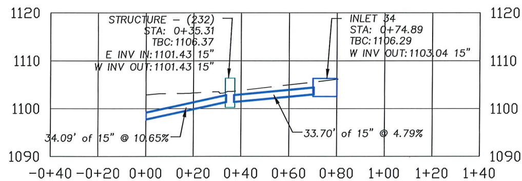
3 ROLLA STREET STORM PROFILE - Rolla St and 9th St Scale: 1" = 40' H
