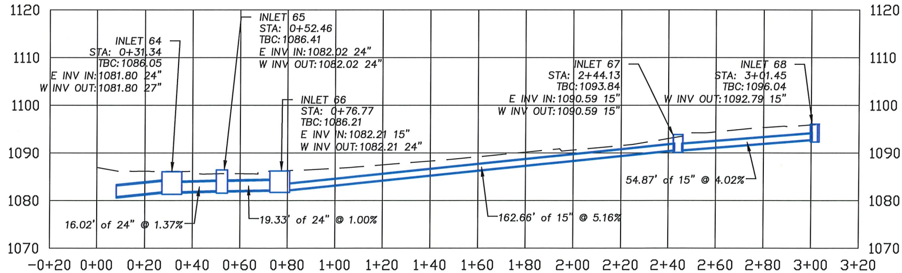
2 ROLLA STREET STORM PROFILE - 6th St from Rolla St to Pine St Scale: 1" = 40' H 1" = 20' V
