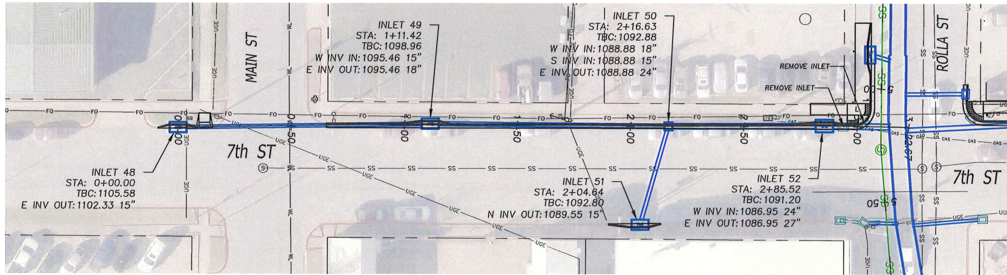
1 ROLLA STREET STORM PLAN - 7th St from Main St to Rolla St 11 Scale: 1" = 40' H
