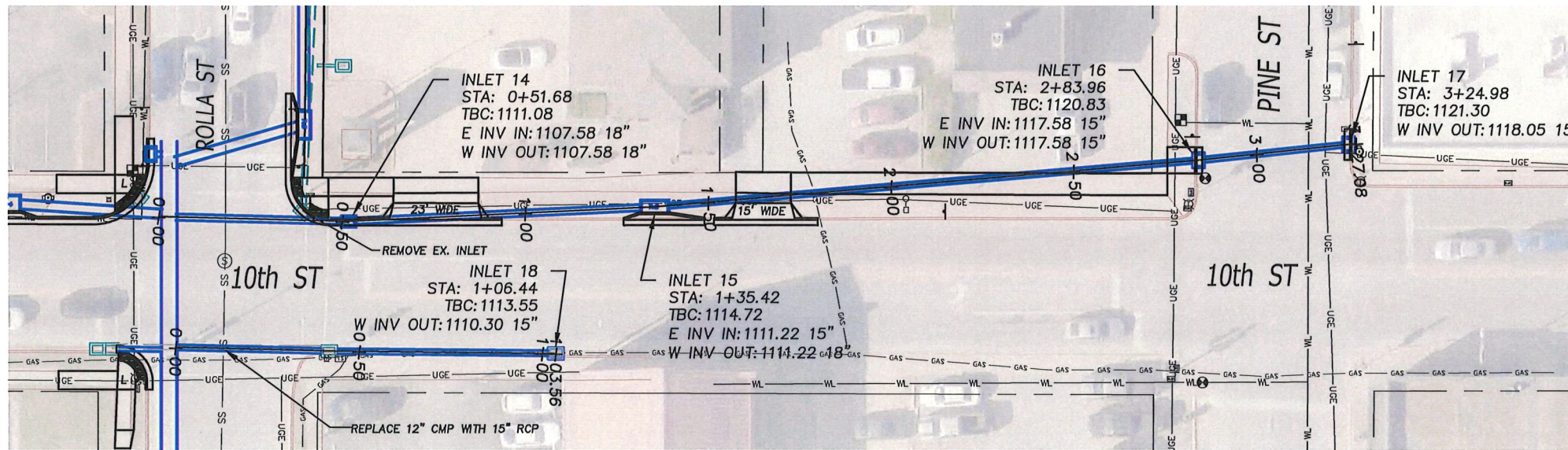
1 ROLLA STREET STORM PLAN - 10th St from Rolla St to Pine St Scale: 1" = 40' H
