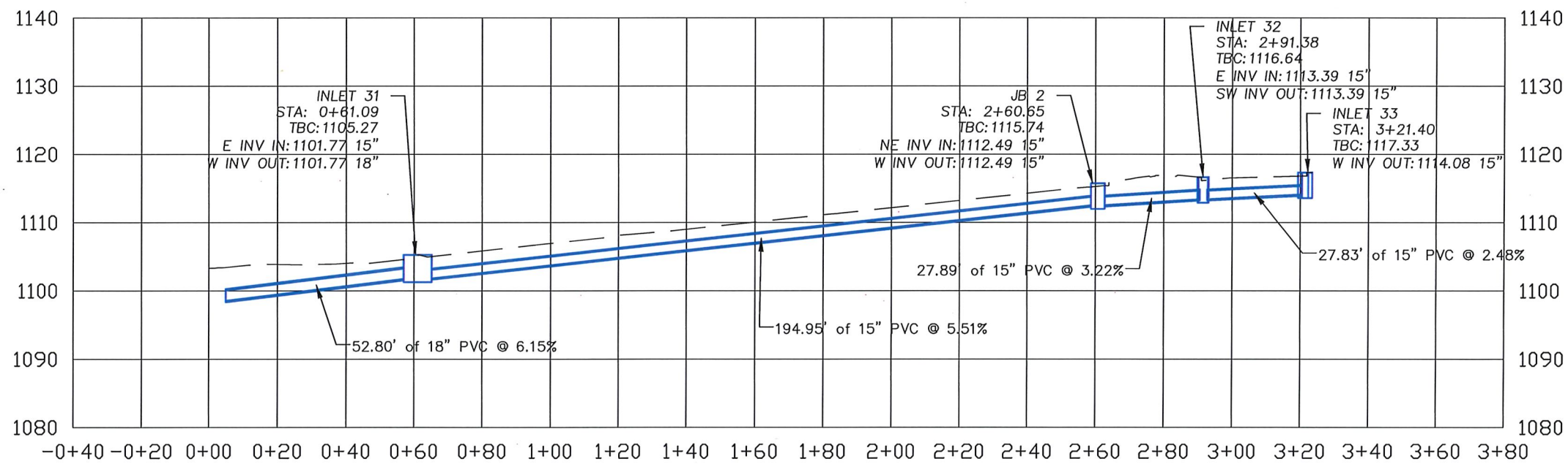
2 ROLLA STREET STORM PROFILE - 9th St from Rolla St to Pine St Scale: 1" = 40' H
