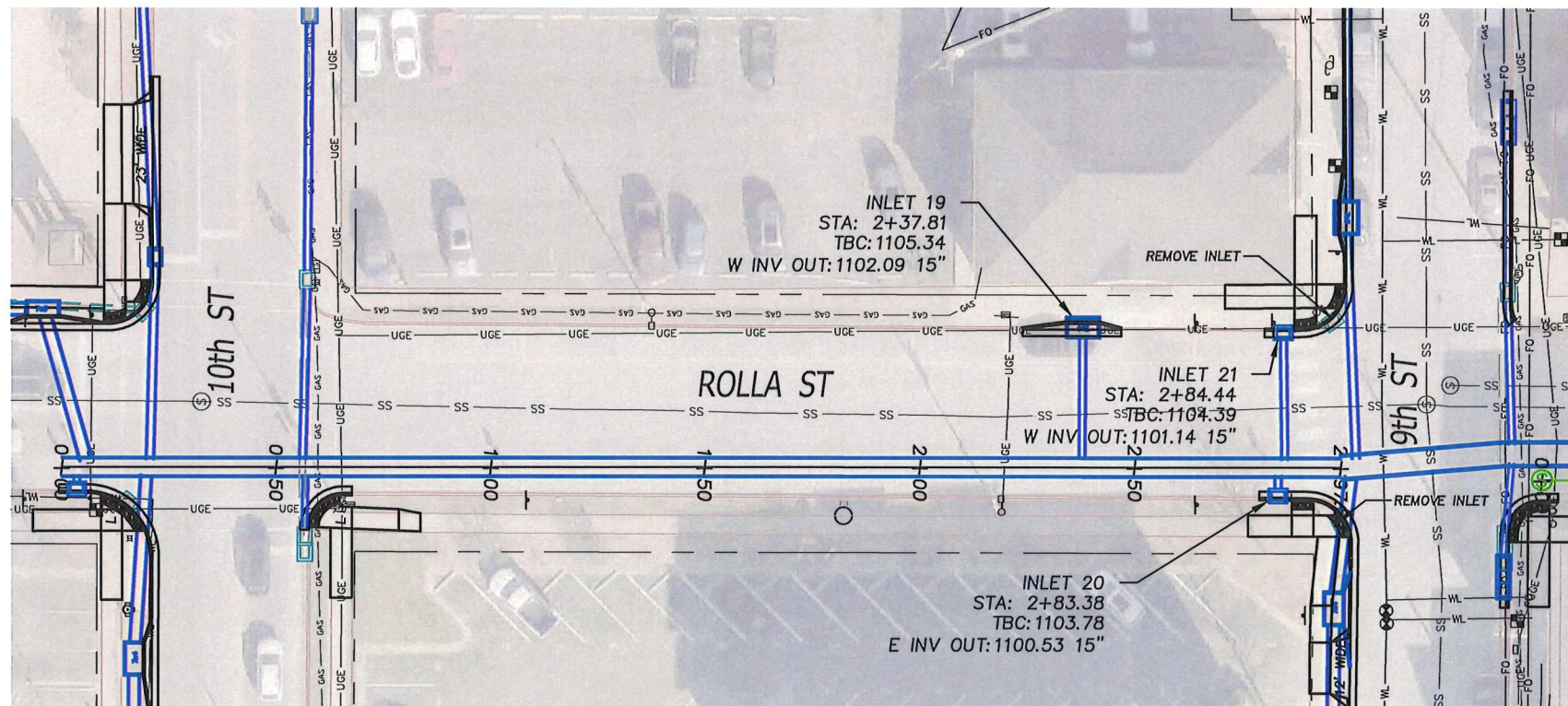
1 5 ROLLA STREET STORM PLAN - Rolla St from 9th St to 10th St Scale: 1" = 40' H
