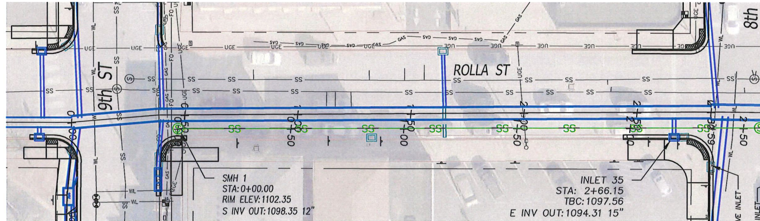
1 8 ROLLA STREET STORM PLAN - Rolla St from 8th St to 9th St Scale: 1" = 40' H
