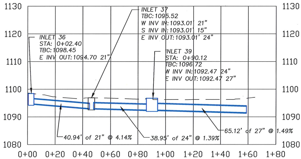
2 9 ROLLA STREET STORM PROFILE - Rolla St and 8th St Scale: 1" = 40' H 1" = 20' V
