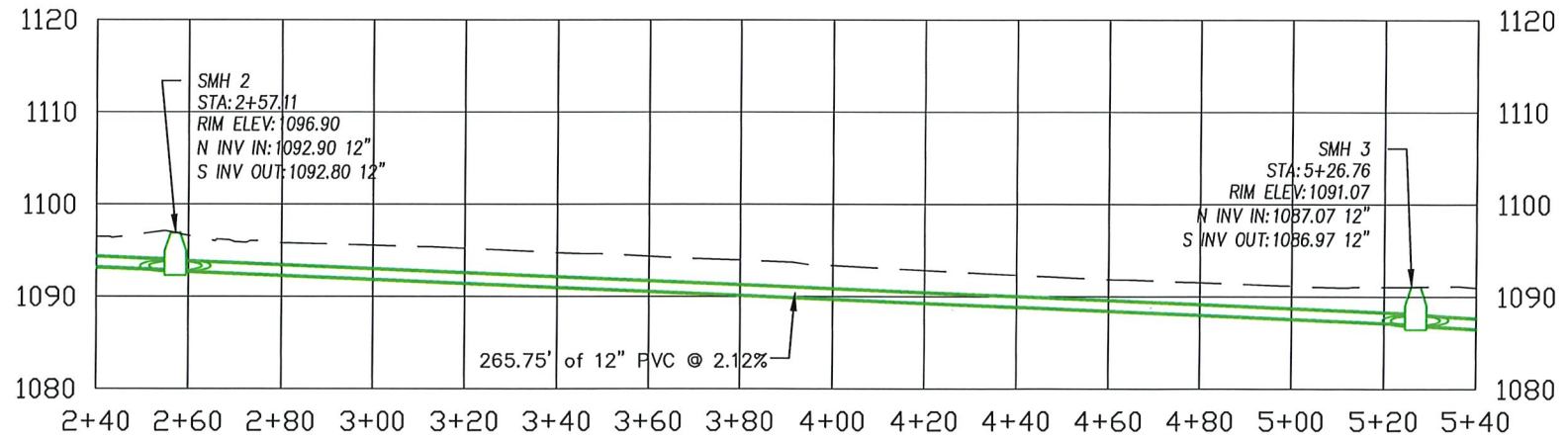
3 ROLLA STREET SANITARY PROFILE - Rolla St from 7th St to 8th St Scale: 1" = 40' H 1" = 20' V
