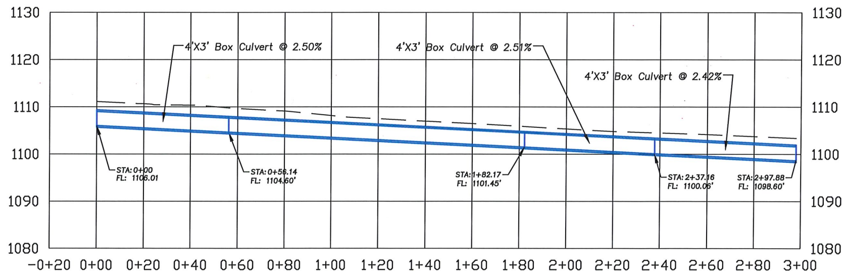
2 5 ROLLA STREET STORM PROFILE - Rolla St from 9th St to 10th St Scale: 1" = 40' H 1" = 20' V
