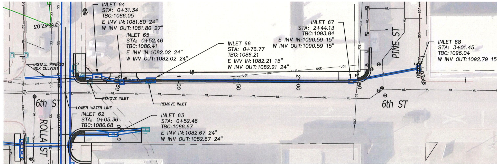
1 ROLLA STREET STORM PLAN - 6th St from Rolla St to Pine St Scale: 1" = 40' H
