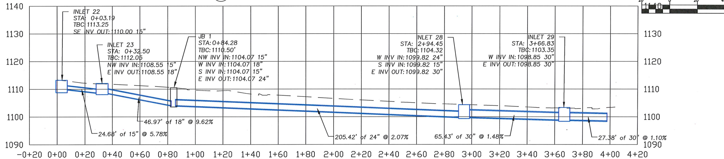
2 ROLLA STREET STORM PLAN - 9th St from Main St to Rolla St Scale: 1" = 40' H
