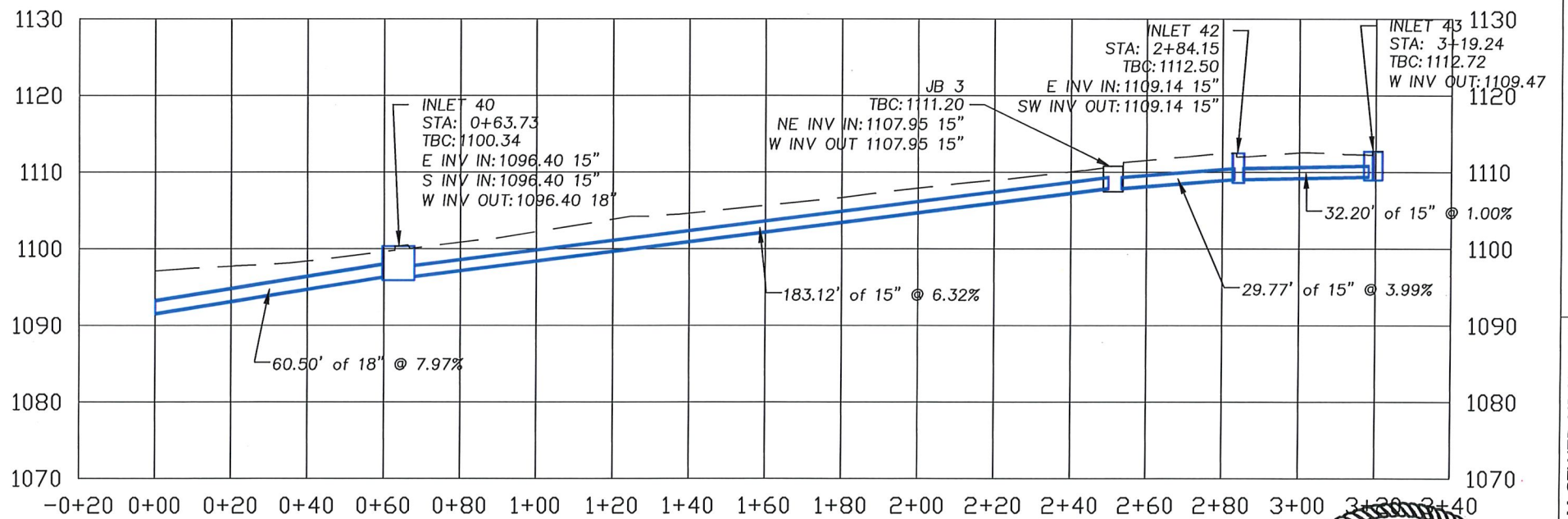
3 9 ROLLA STREET STORM PROFILE - 8th St from Rolla St to Pine St Scale: 1" = 40' H 1" = 20' V
