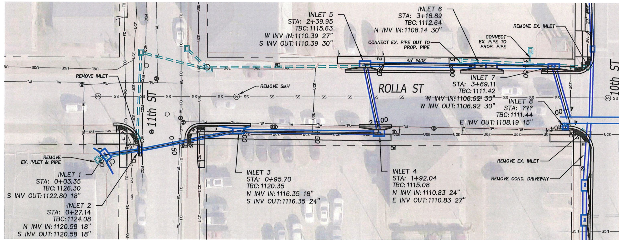
1 ROLLA STREET STORM PLAN - 10th St to 11th St 2 Scale: 1" = 40' H
