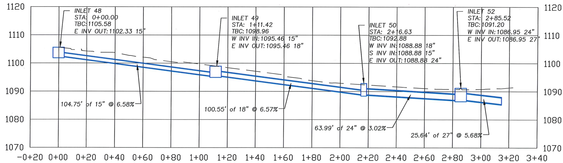
2 ROLLA STREET STORM PROFILE - 7th St from Main St to Rolla St 11 Scale: 1" = 40' H 1" = 20' V
