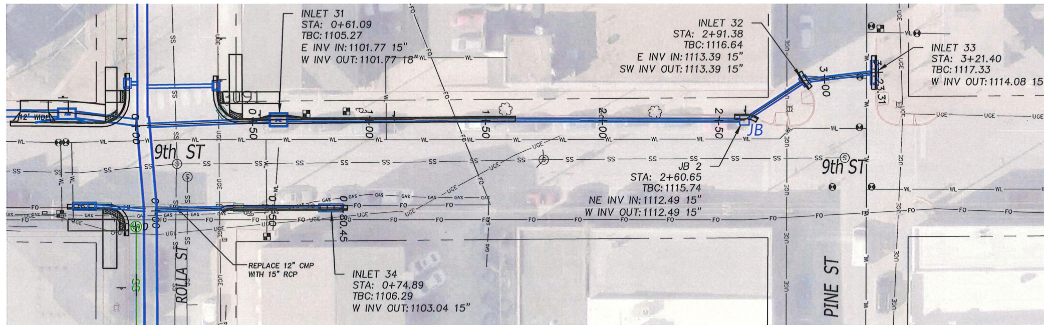
1 ROLLA STREET STORM PLAN - 9th St from Rolla St to Pine St Scale: 1" = 40' H
