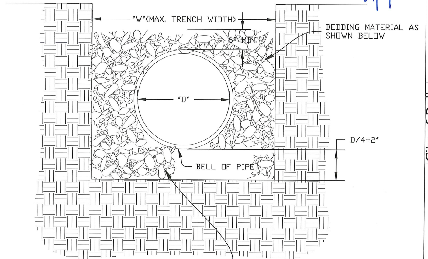
SHAPE BEDDING PRIOR TO INSTALLATION OF PIPE TO A DEPTH OF D/4+2"
