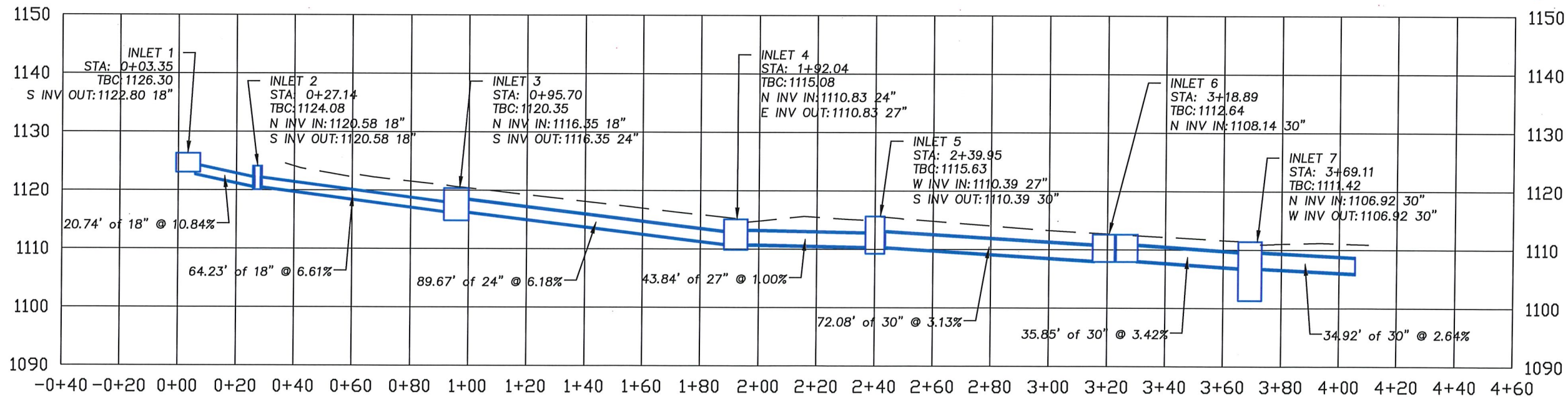
2 ROLLA STREET STORM PROFILE - 10th St to 11th St 2 Scale: 1" = 40' H 1" = 20' V
