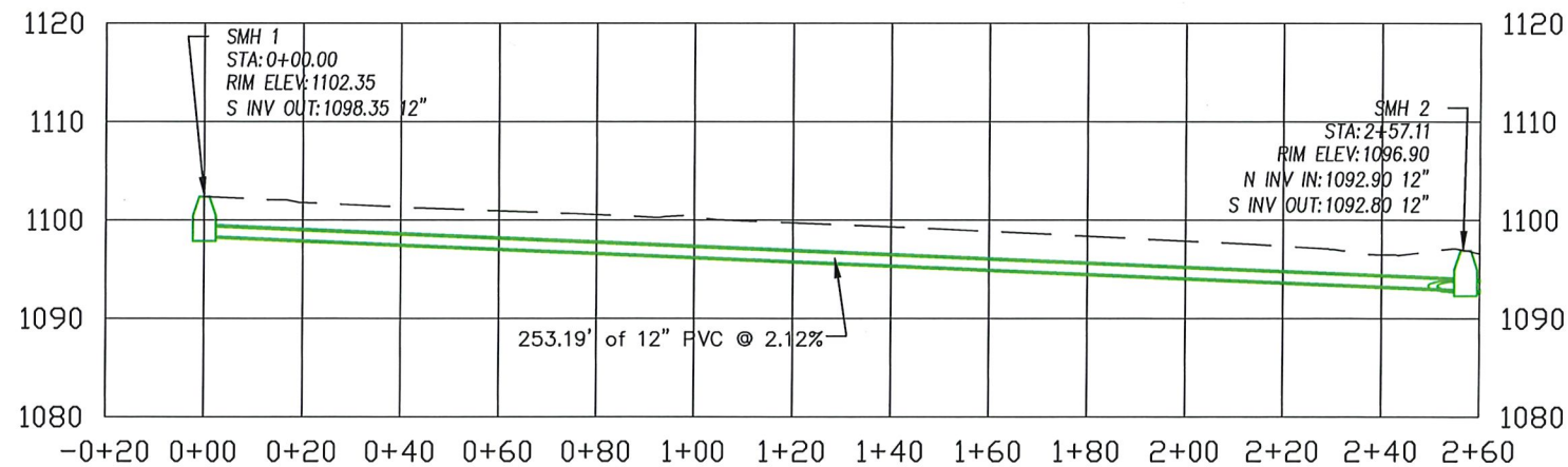
2 8 ROLLA STREET STORM PROFILE - Rolla St from 8th St to 9th St Scale: 1" = 40' H 1" = 20' V
